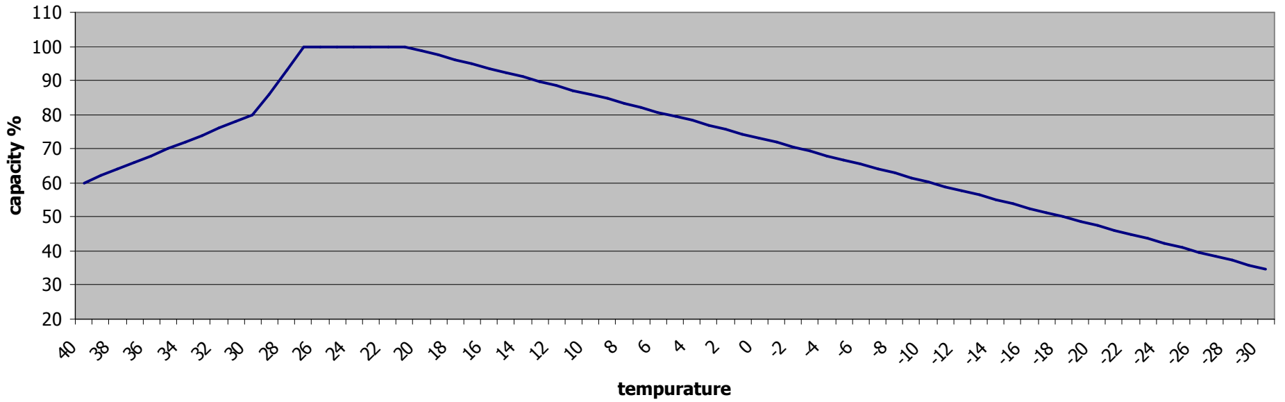
Li-Ion Battery Capacity at Temperature
